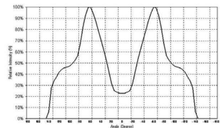
Vertical Spatial Radiation Pattern
