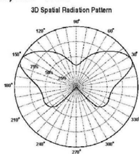
Butterfly-Beam™ Profile
